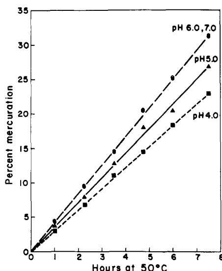
FIGURE 10: Mercuration of poly(U) in 0.1 M sodium acetate buffer: pH 4.0 (■), pH 5.0 (▲), pH 6.0 (●), and pH 7.0 (○). Reactant concentrations and work-up are as described in Figure 6.
