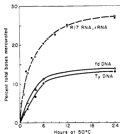
FIGURE 11: Mercuration of R17 RNA (■), 23S rRNA (○), fd DNA (Δ), and native T 7 DNA (●). Each 1.0-ml reaction, run in triplicate, contained 0.005 M sodium acetate buffer (pH 6.0) and 4 \times 10^{-3} M [ ^{203}\text{Hg} ]mercuric acetate ( 1.6 \times 10^7 cpm/ \mu\text{mol} ). The polymer nucleotide concentrations were: rRNA and R17 RNA, 4.0 \times 10^{-4} M ; fd DNA, 4.4 \times 10^{-4} M , and T 7 DNA, 6.1 \times 10^{-4} M . Concentrations were based on 108 nmol/OD 260 nm for rRNA, R17, and fd DNA and 142 nmol/OD 260 for native T 7 DNA. Aliquots were removed at the indicated times and processed, with polymer-free controls, as previously described (Figure 6).
