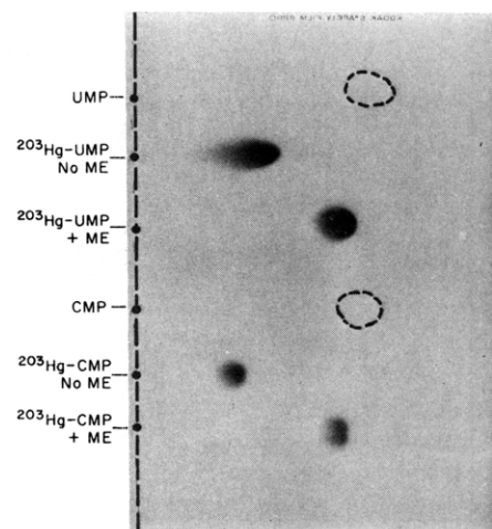
FIGURE 5: Electrophoretic mobility of [ 203 Hg]UMP and Hg-CMP at pH 7.5 in the presence and absence of mercaptoethanol; 0.1 OD 260 of [ 203 Hg]UMP and [ 203 Hg]CMP (containing 1.1 \times 10^5 and 4.5 \times 10^4 cpm, respectively) were applied to a 20 × 20 cm thin-layer cellulose plate and electrophoresed for 1.5 hr at 300 V. The plate was dried and exposed to Kodak RP/R54 film for 2 hr before development. UMP and CMP markers were localized by uv adsorption.
