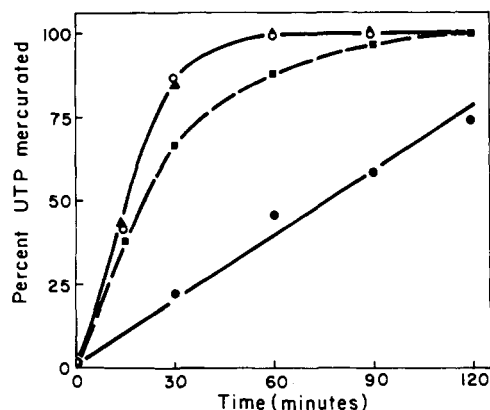
FIGURE 1: Kinetics of UTP mercuration in 0.1 M sodium acetate buffer: pH 4.0 (●), pH 5.0 (■), pH 6.0 (○), and pH 7.0 (▲). Each reaction (10 ml), run in duplicate, contained 6 \times 10^{-4} M UTP and 4 \times 10^{-3} M [ ^{203}\text{Hg} ]mercuric acetate (specific activity, 1.7 \times 10^6 cpm/ \mu\text{mol} ); 1.0-ml aliquots were removed at the indicated times and processed as described under Materials and Methods.
