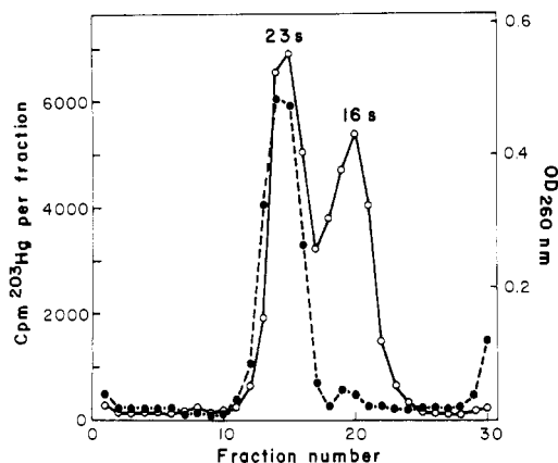
FIGURE 13: Sedimentation profile of 23S rRNA after mercuration of 18% of its pyrimidine bases. Five OD 260 of 23S RNA was treated with [ 203 Hg]mercuric acetate for 90 min under the conditions given in Figure 11. The reaction was quenched and chromatographed on Sephadex G-25 as described in Table V to remove excess mercuric acetate. 0.1 ml of the RNA peak containing 0.15 OD 260 (24,000 cpm of 203 Hg) was removed, 4.0 OD 260 (50 μl) of cold (23S + 16S) rRNA added, and the sample centrifuged in a 5–20% sucrose gradient (in 0.01 M Tris-HCl buffer (pH 7.5)–0.1 M NaCl–10 −5 M mercaptoethanol), for 2.5 hr at 48,000 rpm in an SW 50.1 rotor; 0.15-ml fractions were collected by bottom puncture, 50 μl was counted in 3.0 ml of Aquasol for 203 Hg cpm, and the residual sample was diluted to 1.0 ml with water for OD 260 determinations.
